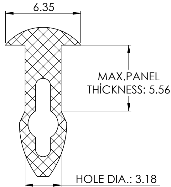
SECTION Y-Y
